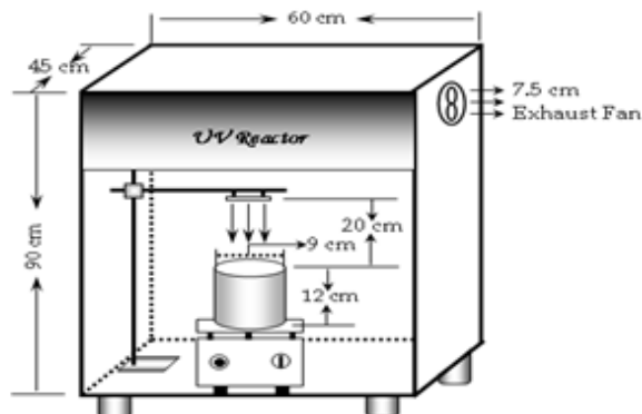
Indigenously designed reactor
