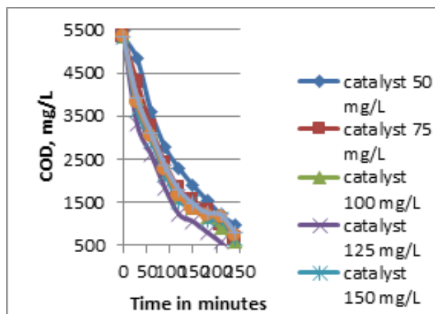
Fig 5: Effect of catalyst concentration on COD removal rate. Detergent concentration = 1000 mg/L, pH = 5.5
