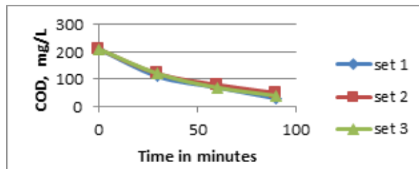
Fig 8: Degradation of sullage under solar radiation. pH = 5.5, temperature = ~30°C, solar radiation ~ 250 W/m², catalyst concentration 125 mg/L, depth of reactor = 15 cm.
