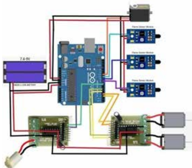
Fig. Circuit Diagram
