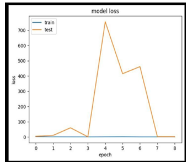
Figure 5 Training process and test model loss Conclusion
