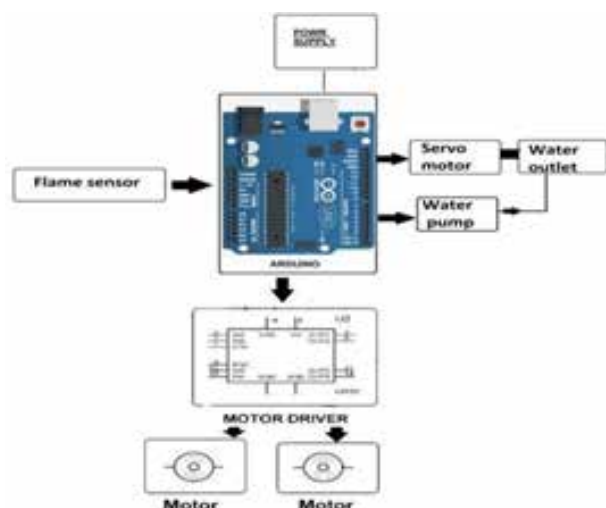
Fig. 1. Block Diagram
