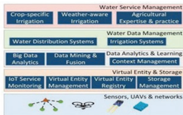
Fig 4. SWAMP architecture
