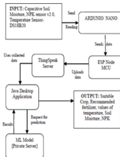
Fig. 1. Block Diagram
