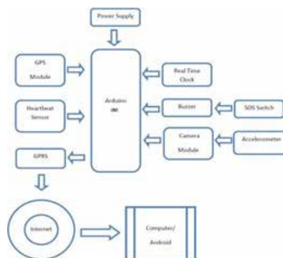
Fig. 7. Block Diagram of Wearable Sensor
