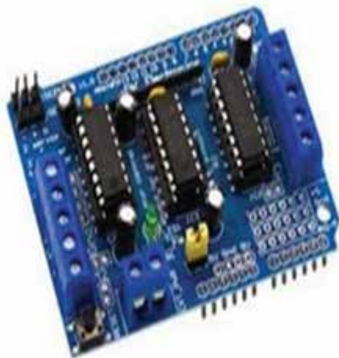
Fig 2: L293D Motor Driver
