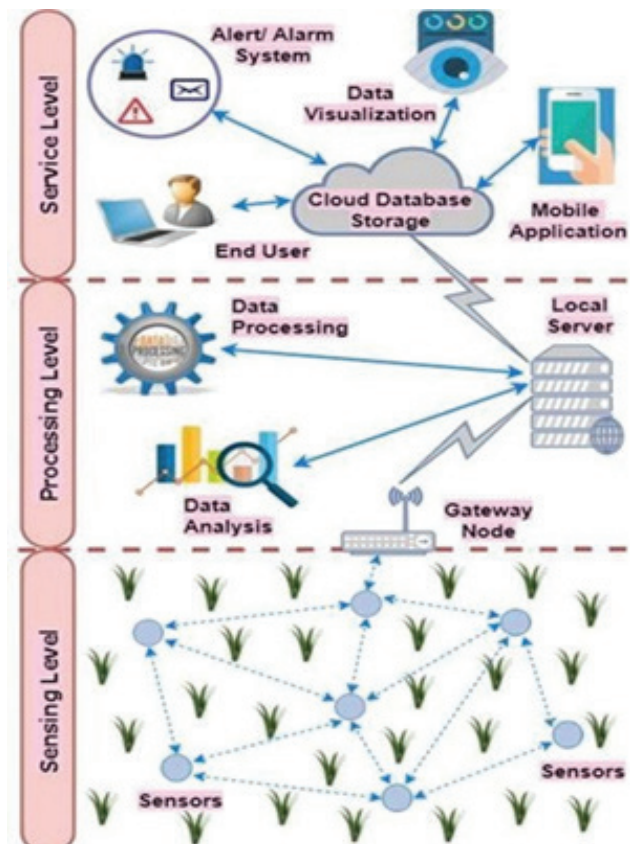
Fig 1. IOT architecture
