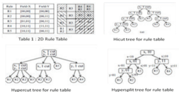
Fig. 2. HiCut, Hypercut and Hypersplit trees for rule set
