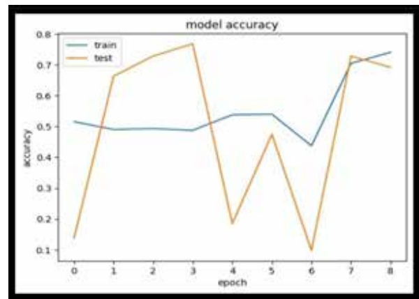
Figure.4 Training process and testing accuracy Degree model
