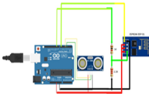
Fig.4 :Circuit diagram of proposed system
