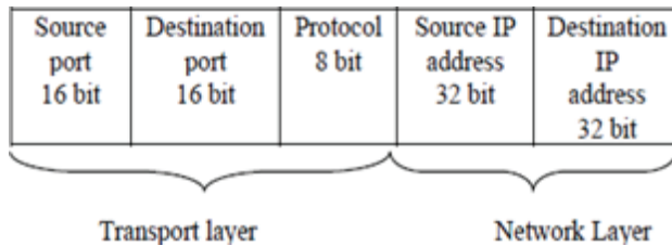
Fig 1. Attributes employed in categorizing packets
